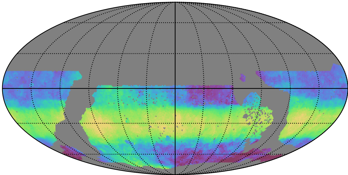
ddf_acor_sf10_lsf20_lsr50_v3.4_10yrs WFD z band: Median HA
