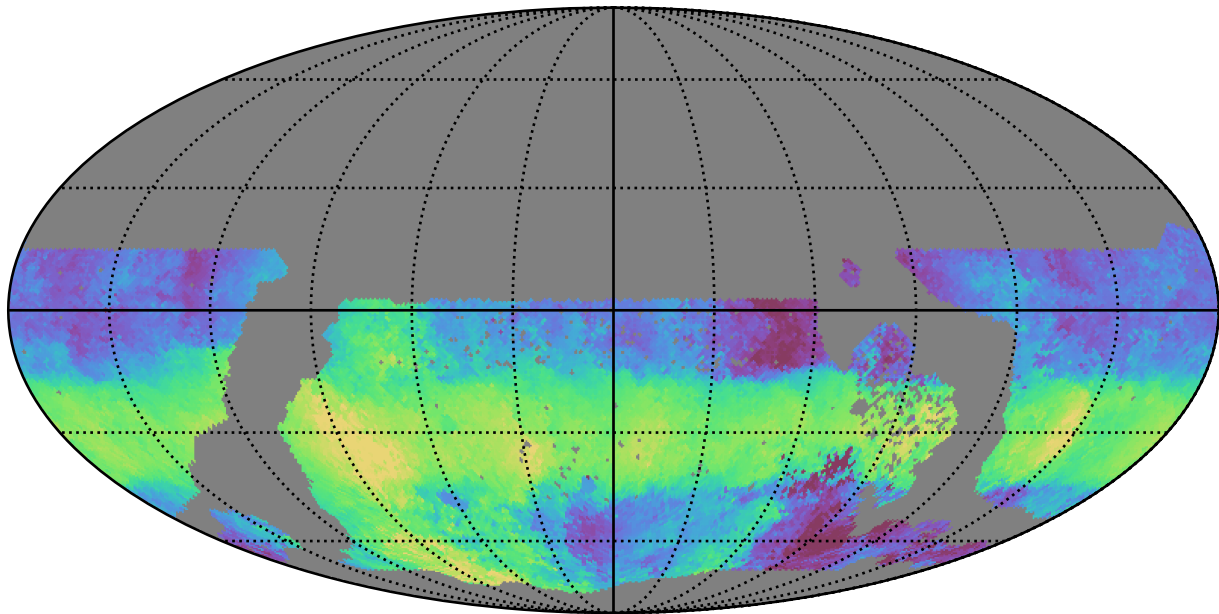
ddf_acor_sf10_lsf20_lsr50_v3.4_10yrs WFD u band: Median HA
