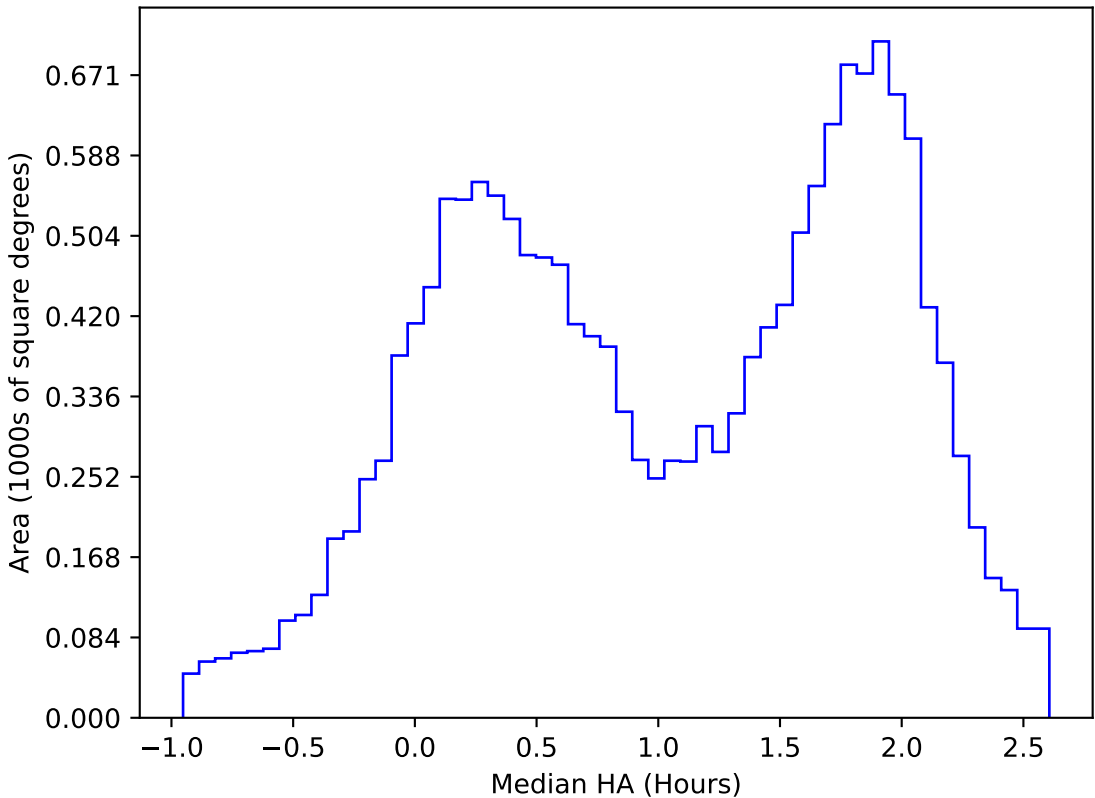
ddf_acor_sf10_lsf20_lsr50_v3.4_10yrs WFD u band: Median HA
