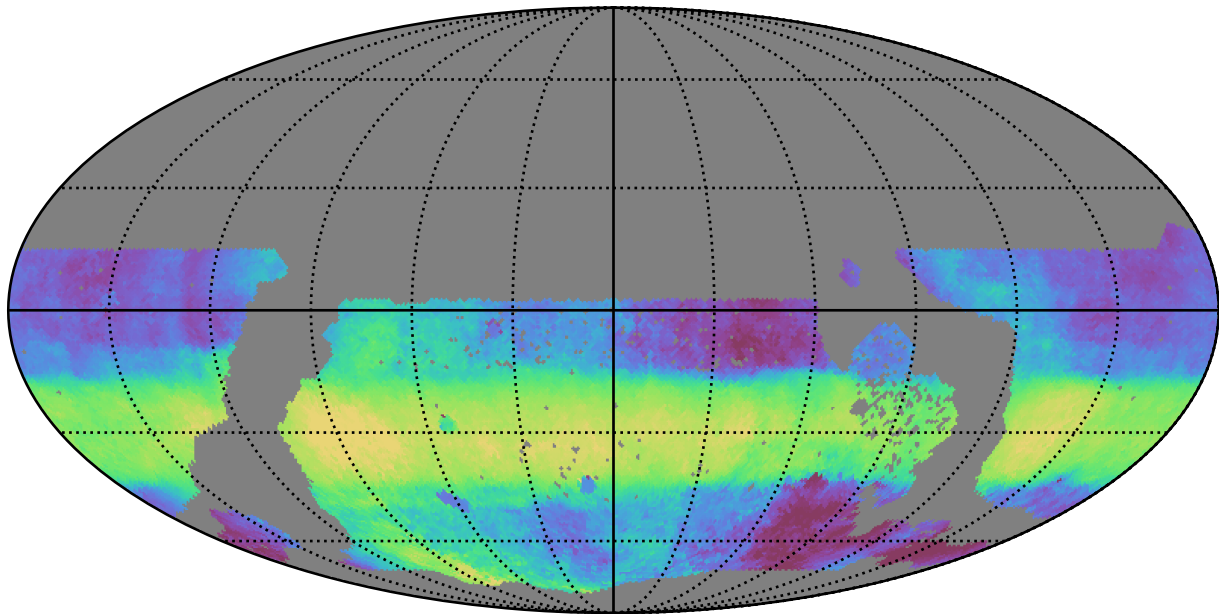
ddf_acor_sf10_lsf20_lsr50_v3.4_10yrs WFD r band: Median HA
