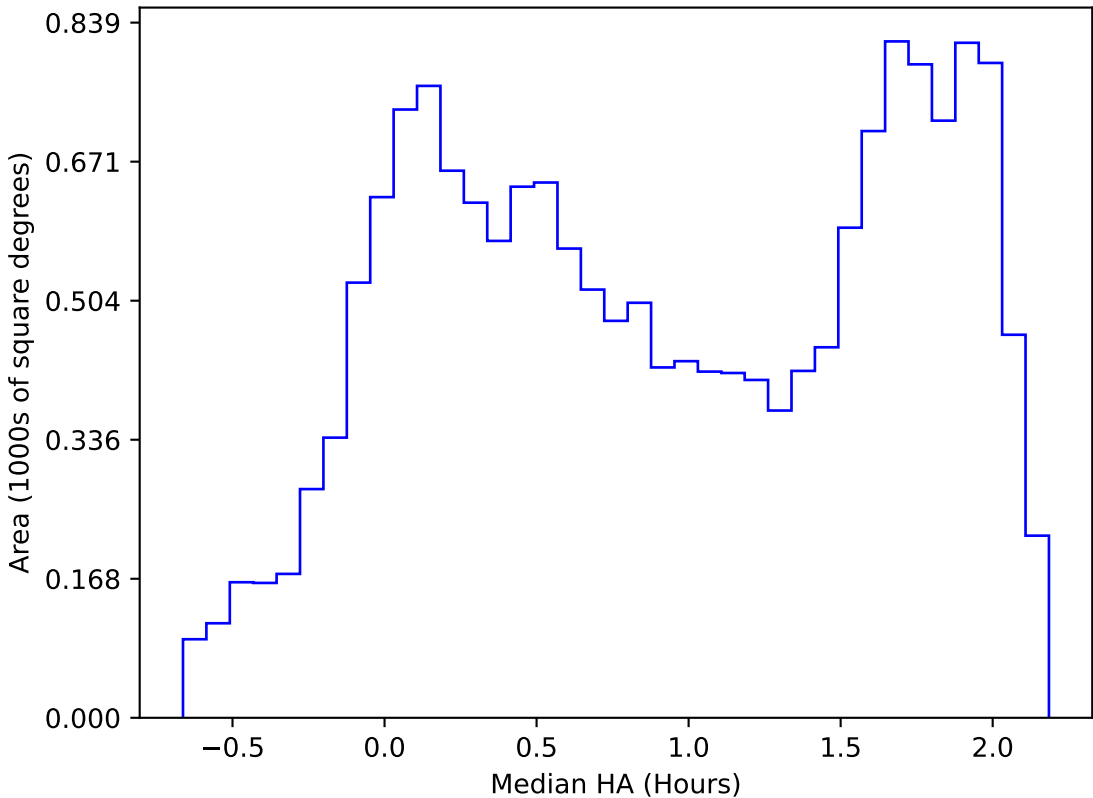
ddf_acor_sf10_lsf20_lsr50_v3.4_10yrs WFD r band: Median HA
