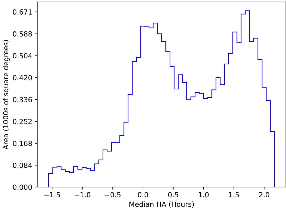
ddf_acor_sf10_lsf20_lsr50_v3.4_10yrs WFD g band: Median HA
