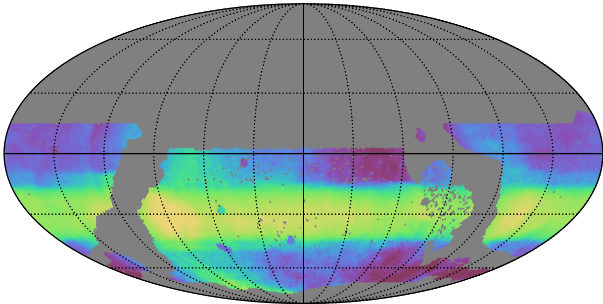
ddf_acor_sf10_lsf20_lsr50_v3.4_10yrs WFD all bands: Median HA
