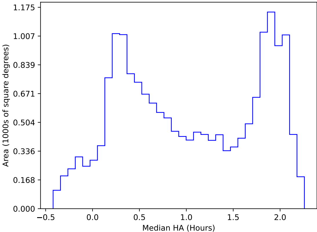
ddf_acor_sf10_lsf20_lsr50_v3.4_10yrs WFD all bands: Median HA
