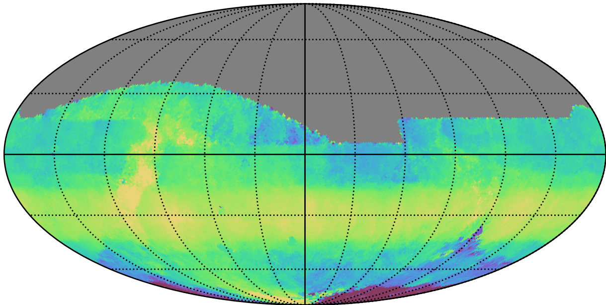
ddf_acor_sf10_lsf20_lsr50_v3.4_10yrs All sky z band: Median HA
