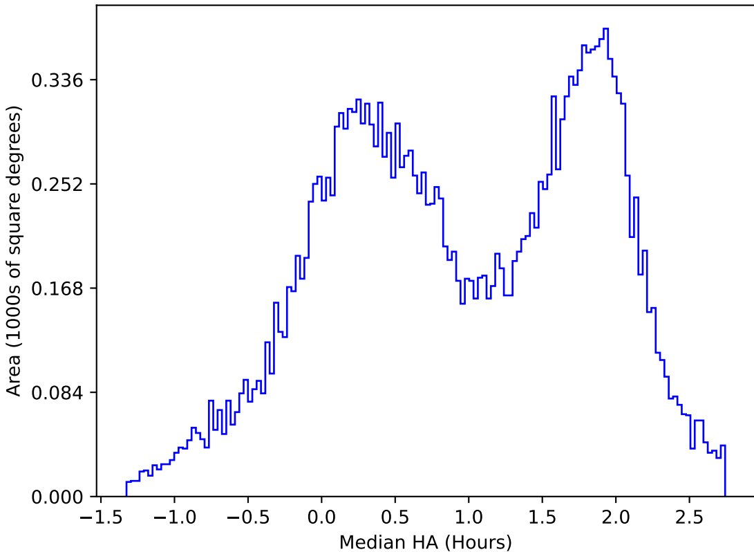
ddf_acor_sf10_ls20_lsr50_v3.4_10yrs All sky u band: Median HA
