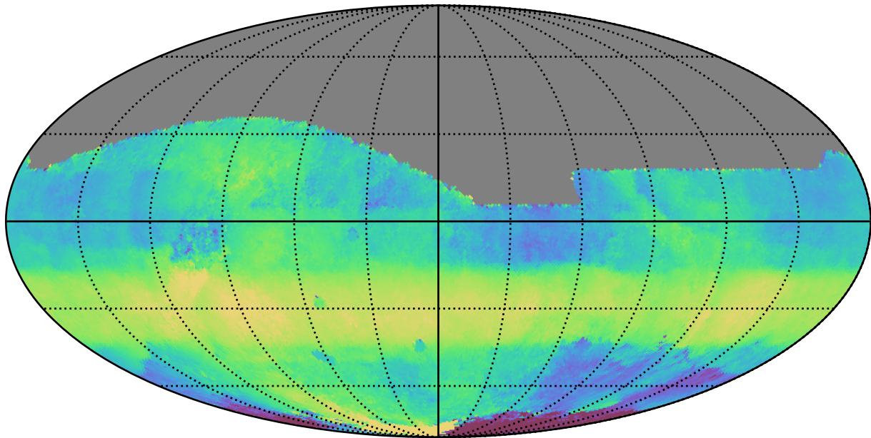
ddf_acor_sf10_lsf20_lsr50_v3.4_10yrs All sky r band: Median HA
