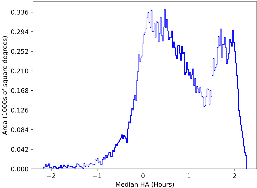
ddf_acor_sf10_lsf20_lsr50_v3.4_10yrs All sky r band: Median HA
