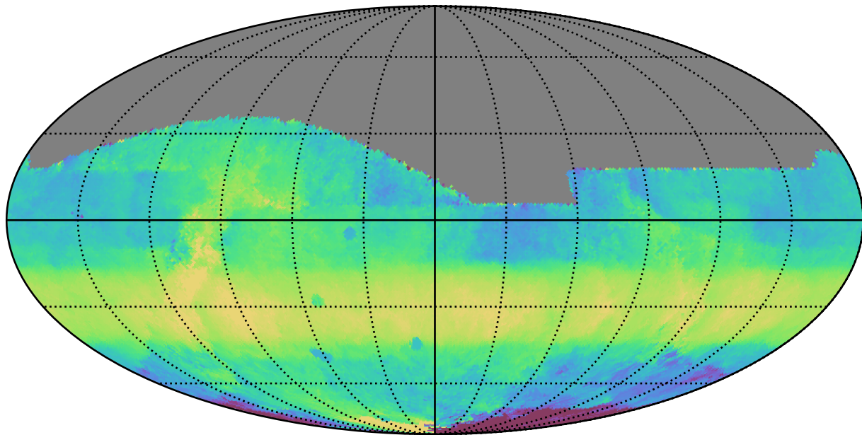
ddf_acor_sf10_lsf20_lsr50_v3.4_10yrs All sky i band: Median HA
