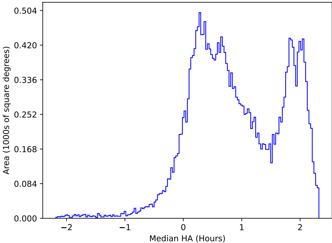
ddf_acor_sf10_lsf20_lsr50_v3.4_10yrs All sky i band: Median HA
