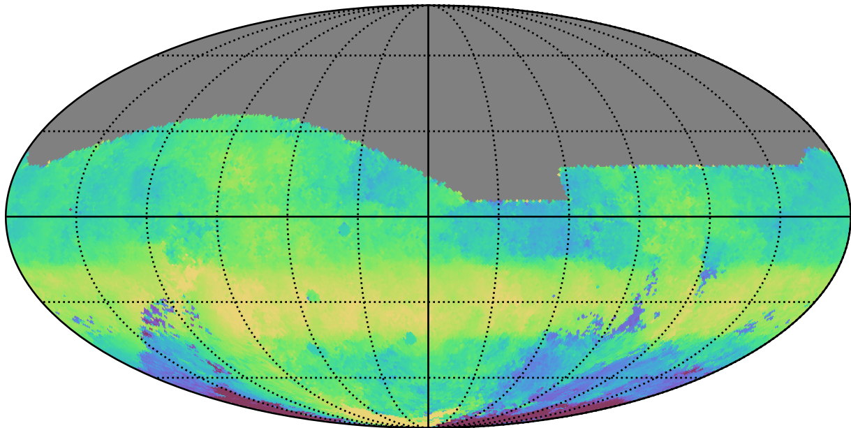
ddf_acor_sf10_lsf20_lsr50_v3.4_10yrs All sky g band: Median HA
