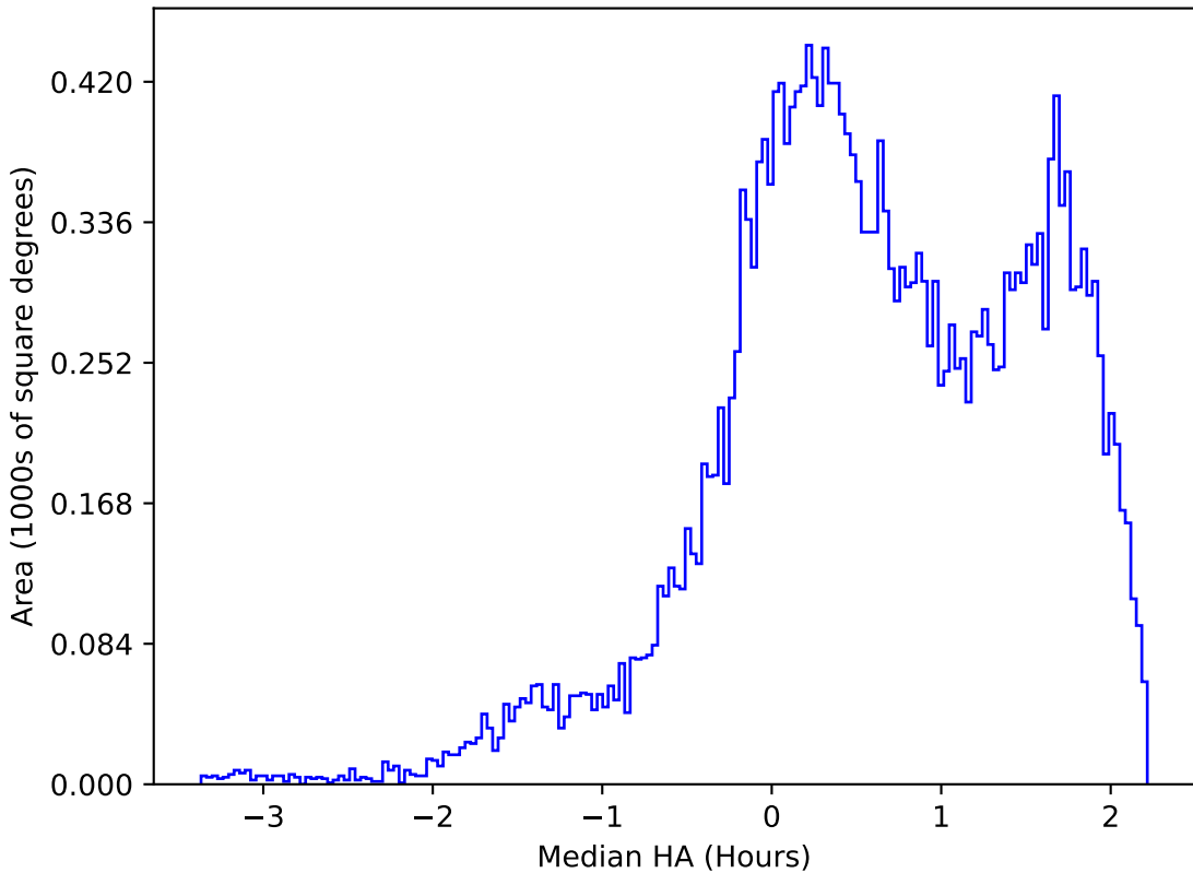
ddf_acor_sf10_lsf20_lsr50_v3.4_10yrs All sky g band: Median HA
