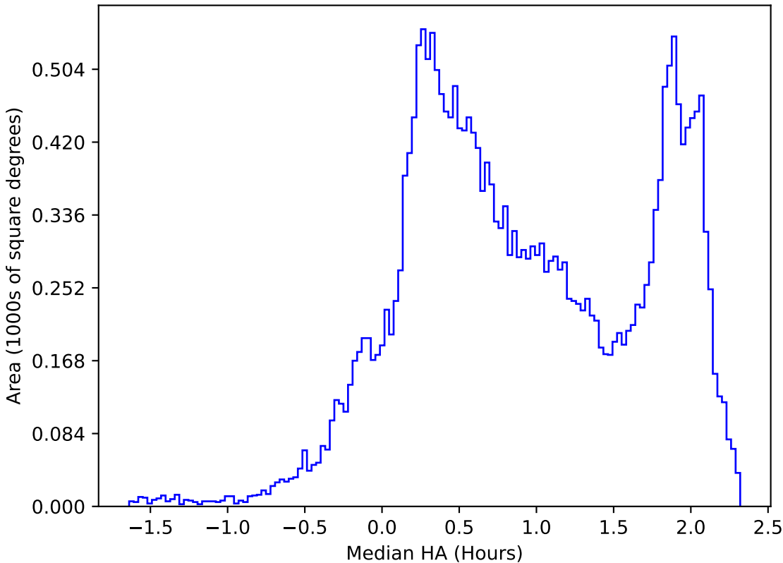
ddf_acor_sf10_lsf20_lsr50_v3.4_10yrs All sky all bands: Median HA
