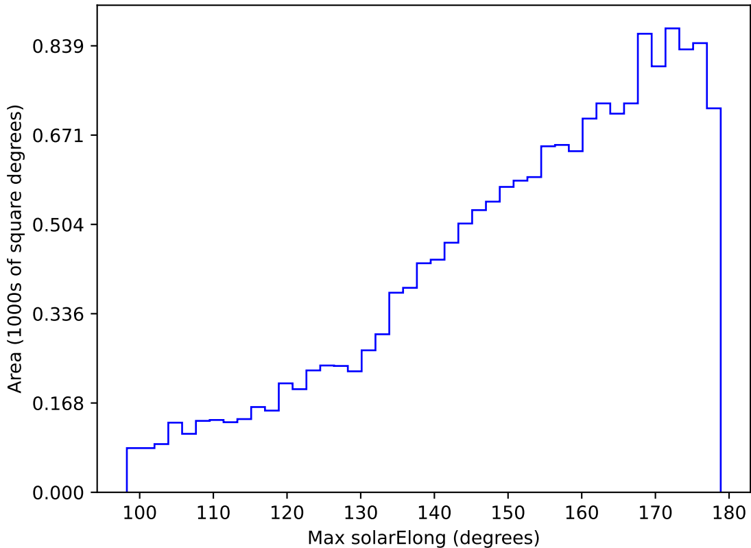
ddf_acor_sf10_lsf20_lsr50_v3.4_10yrs WFD u band: Max solarElong
