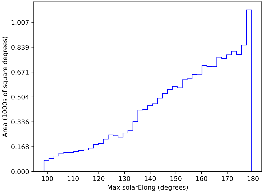
ddf_acor_sf10_lsf20_lsr50_v3.4_10yrs WFD r band: Max solarElong
