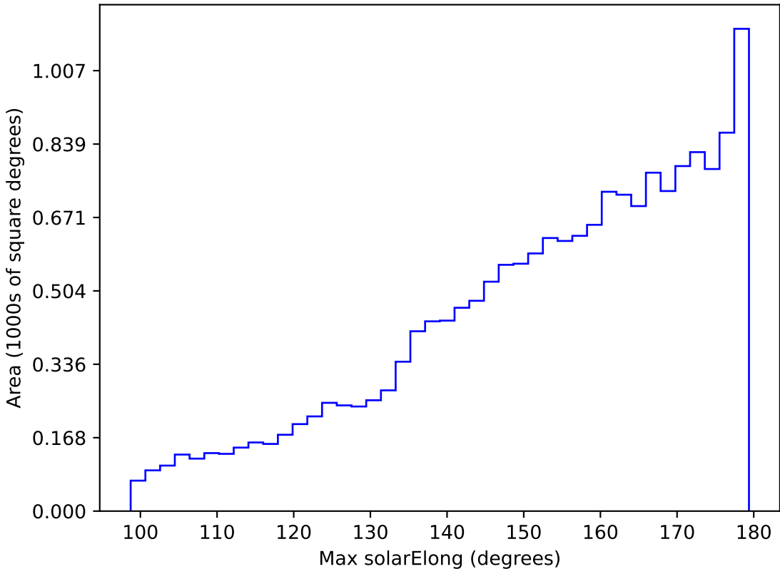
ddf_acor_sf10_lsf20_lsr50_v3.4_10yrs WFD i band: Max solarElong
