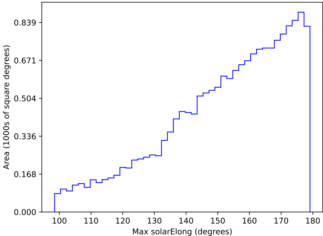
ddf_acor_sf10_lsf20_lsr50_v3.4_10yrs WFD g band: Max solarElong
