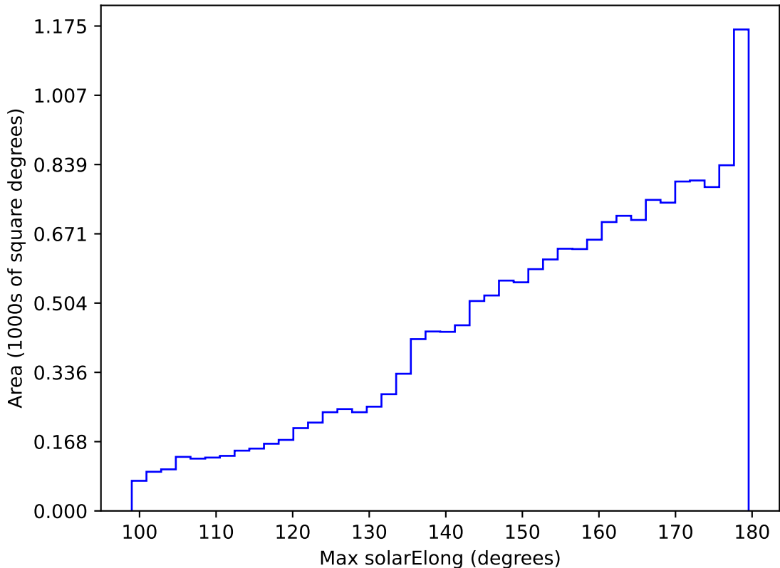
ddf_acor_sf10_lsf20_lsr50_v3.4_10yrs WFD all bands: Max solarElong
