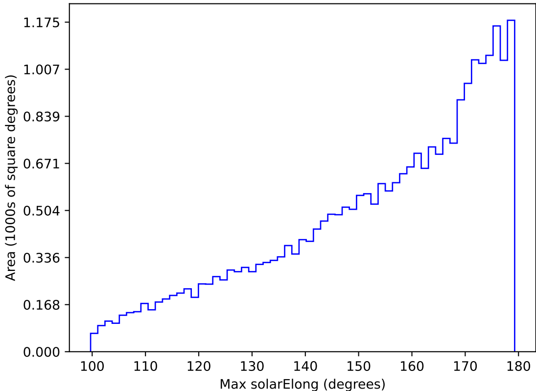
ddf_acor_sf10_lsf20_lsr50_v3.4_10yrs All sky z band: Max solarElong
