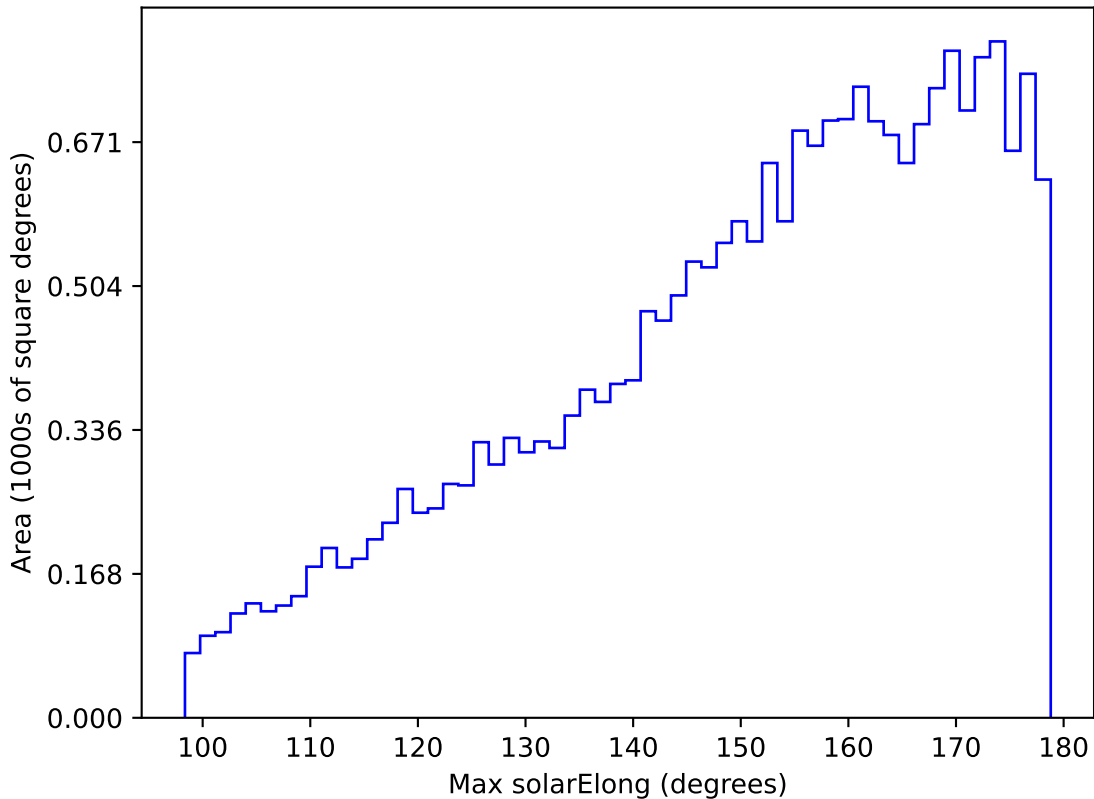
ddf_acor_sf10_lsf20_lsr50_v3.4_10yrs All sky u band: Max solarElong
