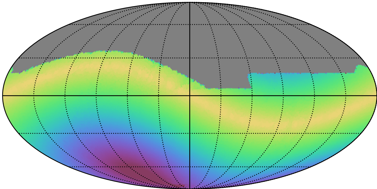
ddf_acor_sf10_lsf20_lsr50_v3.4_10yrs All sky r band: Max solarElong
