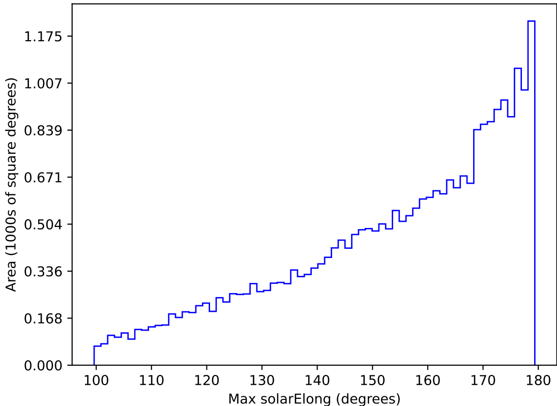
ddf_acor_sf10_lsf20_lsr50_v3.4_10yrs All sky i band: Max solarElong
