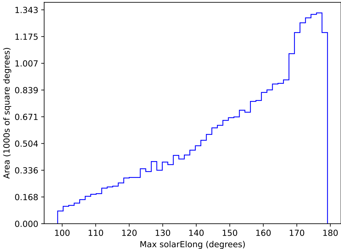
ddf_acor_sf10_lsf20_lsr50_v3.4_10yrs All sky g band: Max solarElong
