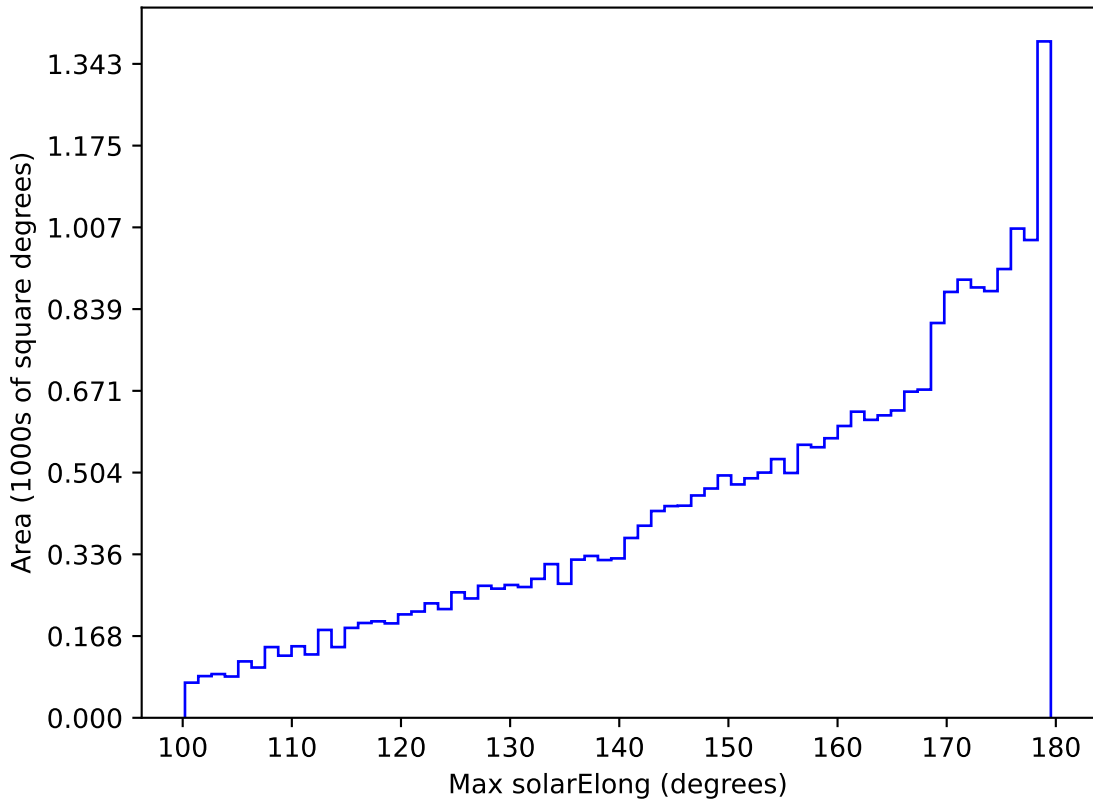
ddf_acor_sf10_lsf20_lsr50_v3.4_10yrs All sky all bands: Max solarElong
