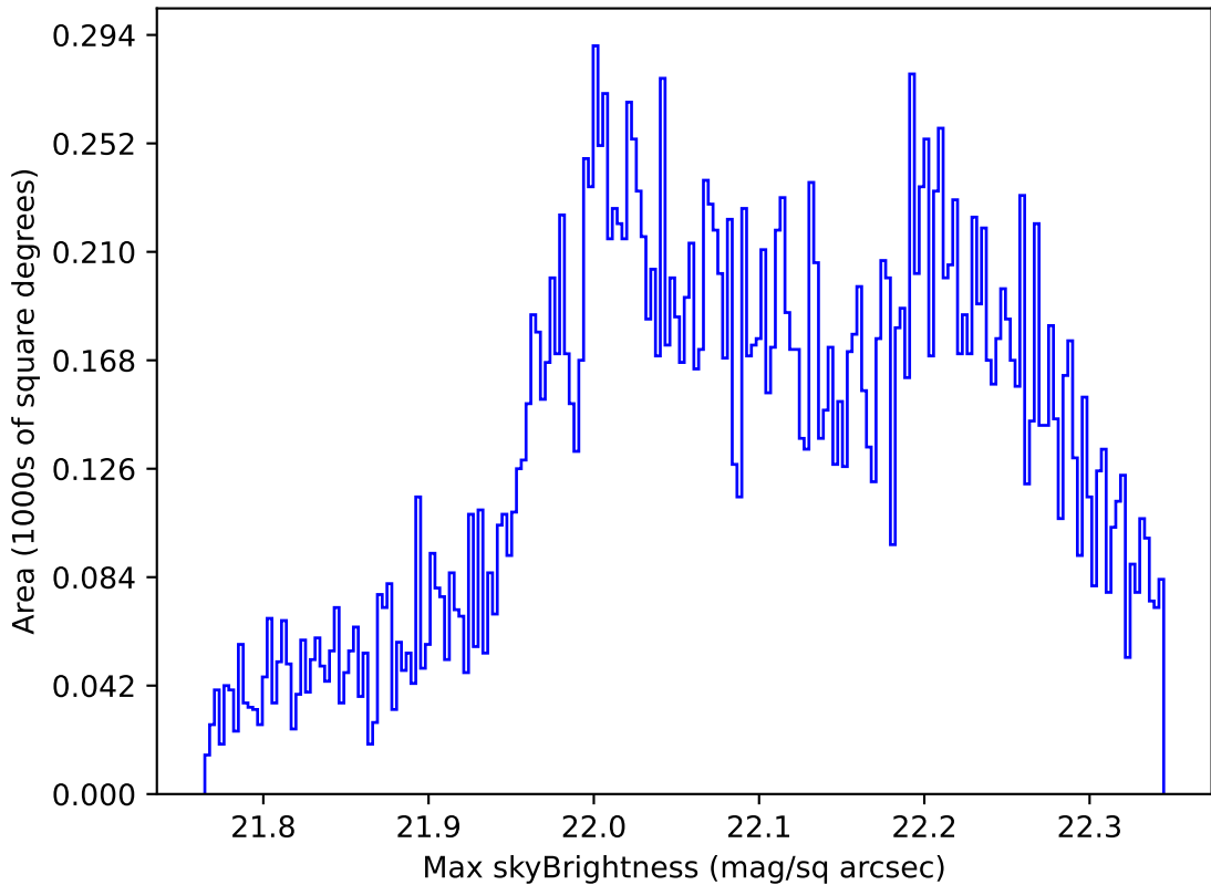
ddf_acor_sf10_lsf20_lsr50_v3.4_10yrs Yr 1 g band: Max skyBrightness
