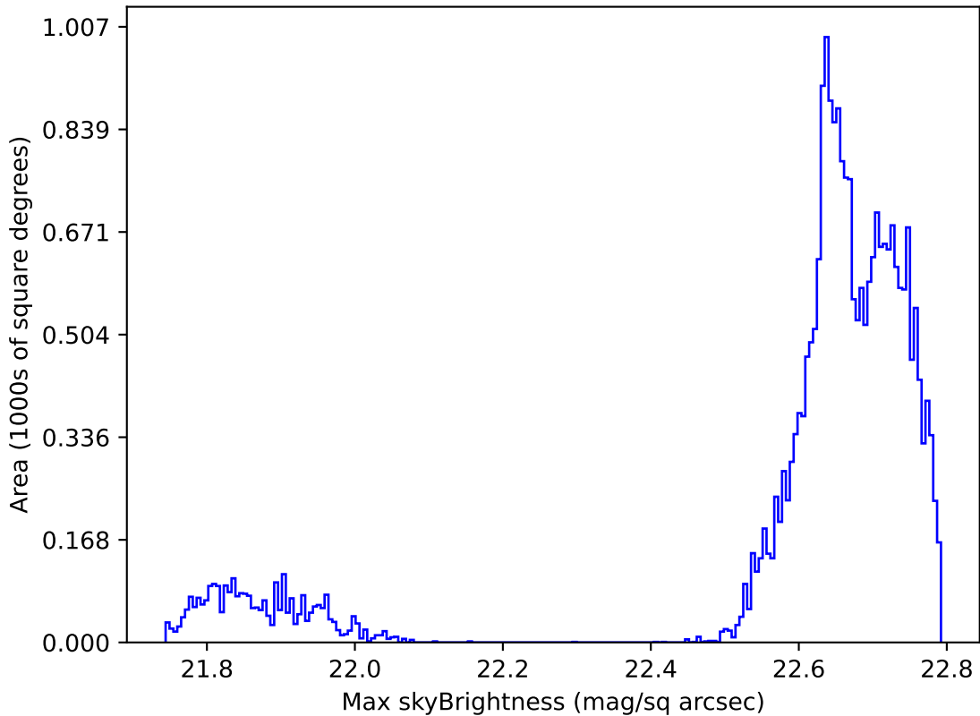
ddf_acor_sf10_lsf20_lsr50_v3.4_10yrs Yr 1 all bands: Max skyBrightness
