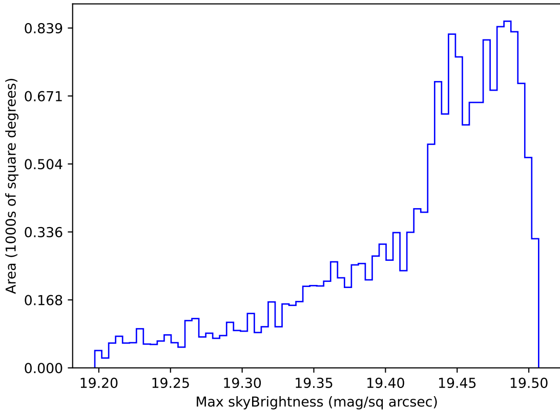
ddf_acor_sf10_lsf20_lsr50_v3.4_10yrs WFD z band: Max skyBrightness
