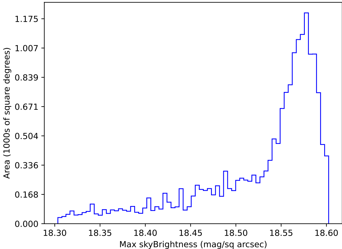
ddf_acor_sf10_lsf20_lsr50_v3.4_10yrs WFD y band: Max skyBrightness
