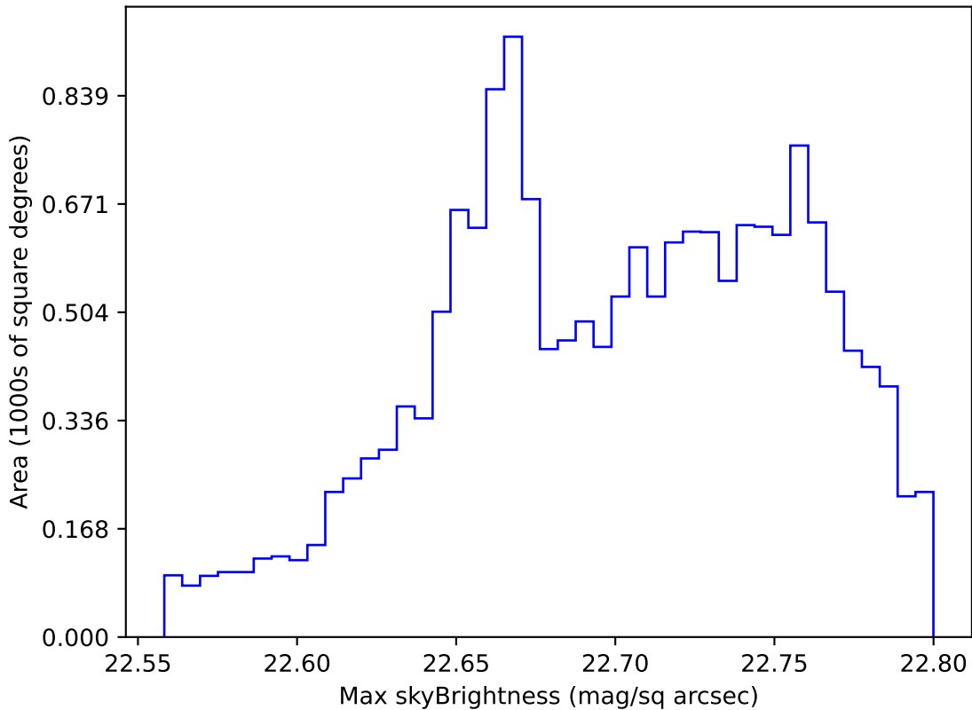
ddf_acor_sf10_lsf20_lsr50_v3.4_10yrs WFD u band: Max skyBrightness
