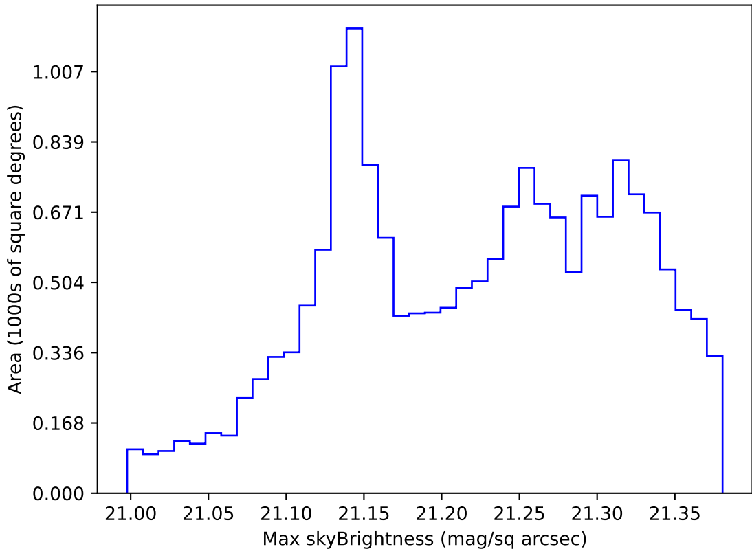
ddf_acor_sf10_lsf20_lsr50_v3.4_10yrs WFD r band: Max skyBrightness
