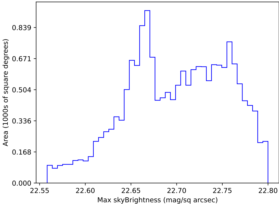
ddf_acor_sf10_lsf20_lsr50_v3.4_10yrs WFD all bands: Max skyBrightness
