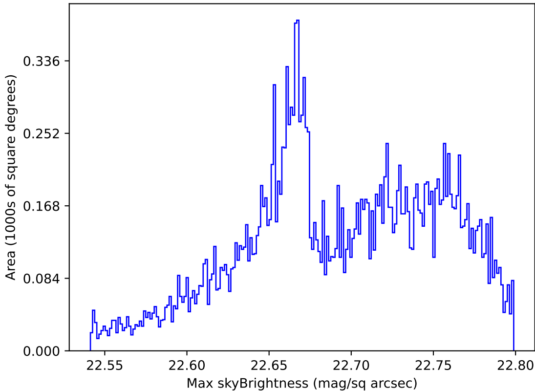
ddf_acor_sf10_lsf20_lsr50_v3.4_10yrs All sky u band: Max skyBrightness
