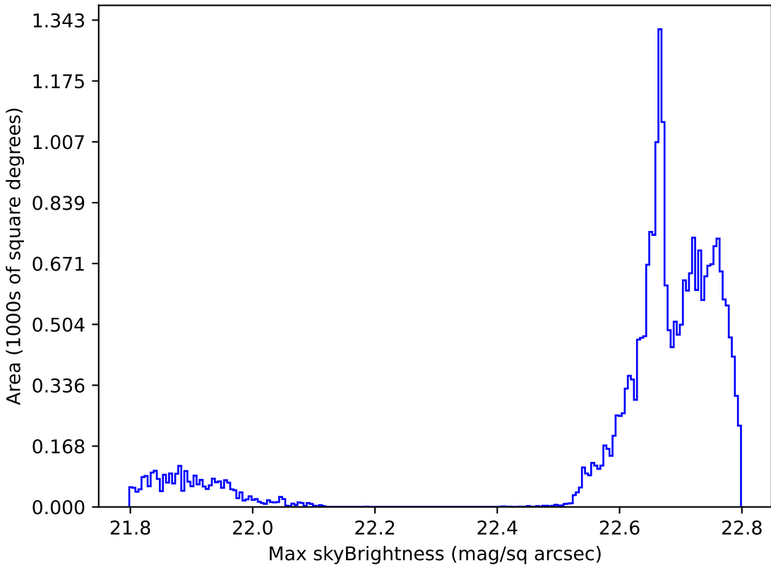
ddf_acor_sf10_lsf20_lsr50_v3.4_10yrs All sky all bands: Max skyBrightness
