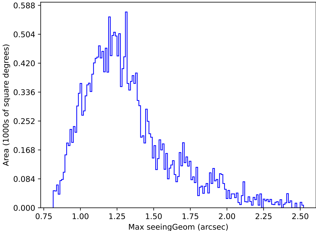
ddf_acor_sf10_lsf20_lsr50_v3.4_10yrs Yr 1 u band: Max seeingGeom
