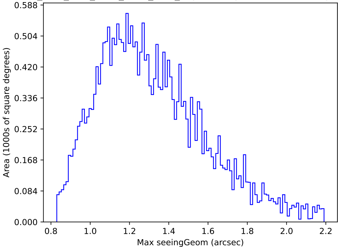
ddf_acor_sf10_lsf20_lsr50_v3.4_10yrs Yr 1 g band: Max seeingGeom
