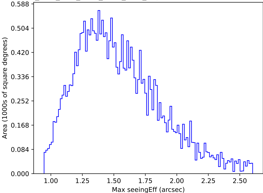
ddf_acor_sf10_lsf20_lsr50_v3.4_10yrs Yr 1 g band: Max seeingEff
