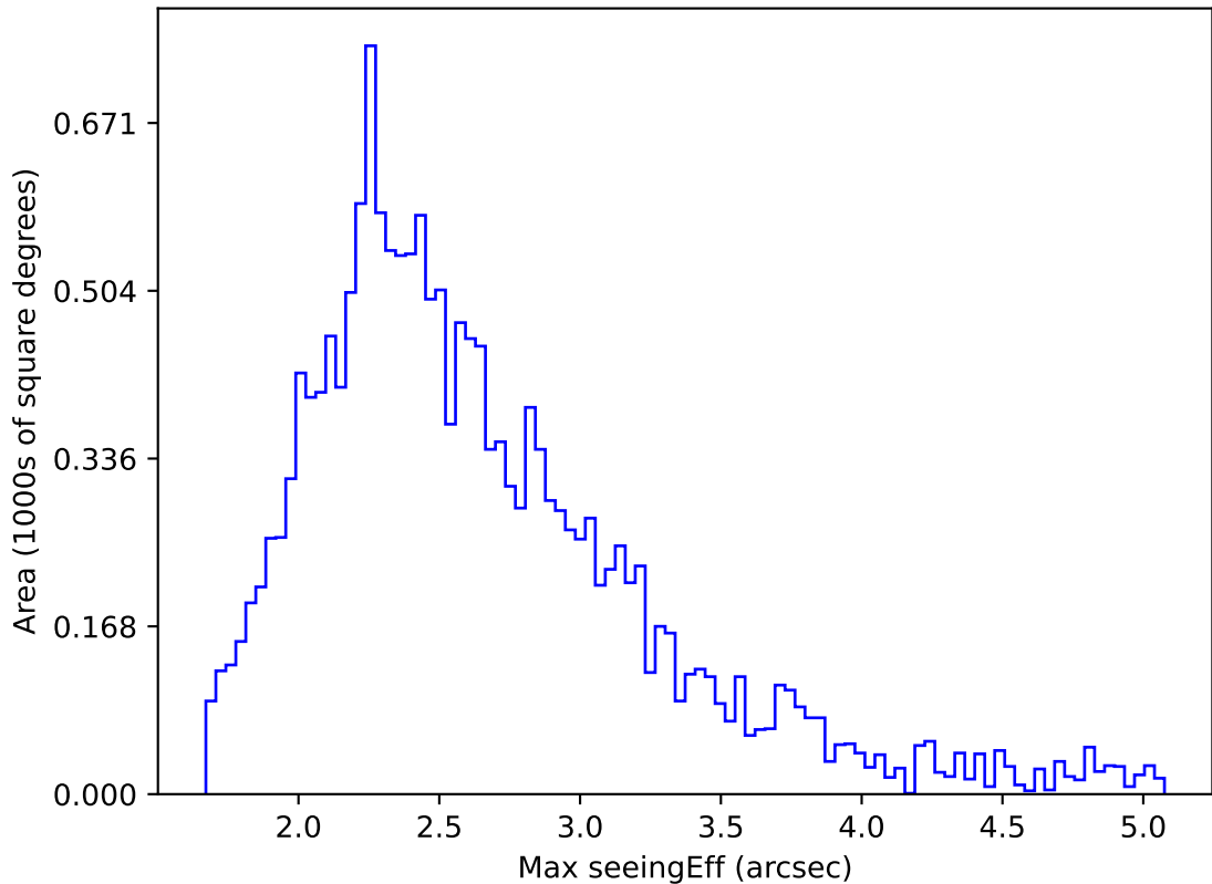
ddf_acor_sf10_lsf20_lsr50_v3.4_10yrs WFD z band: Max seeingEff
