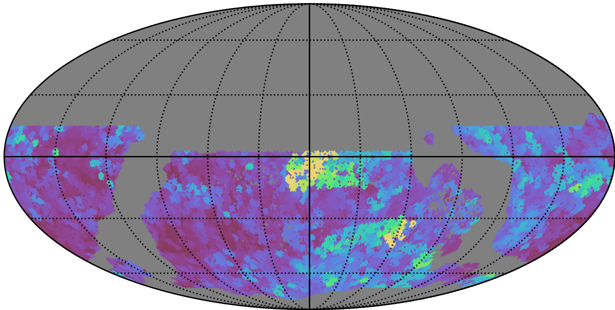
ddf_acor_sf10_lsf20_lsr50_v3.4_10yrs WFD y band: Max seeingEff
