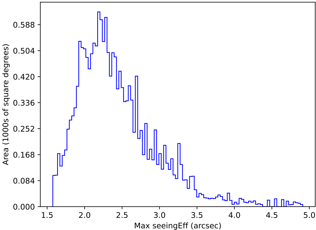
ddf_acor_sf10_lsf20_lsr50_v3.4_10yrs WFD y band: Max seeingEff
