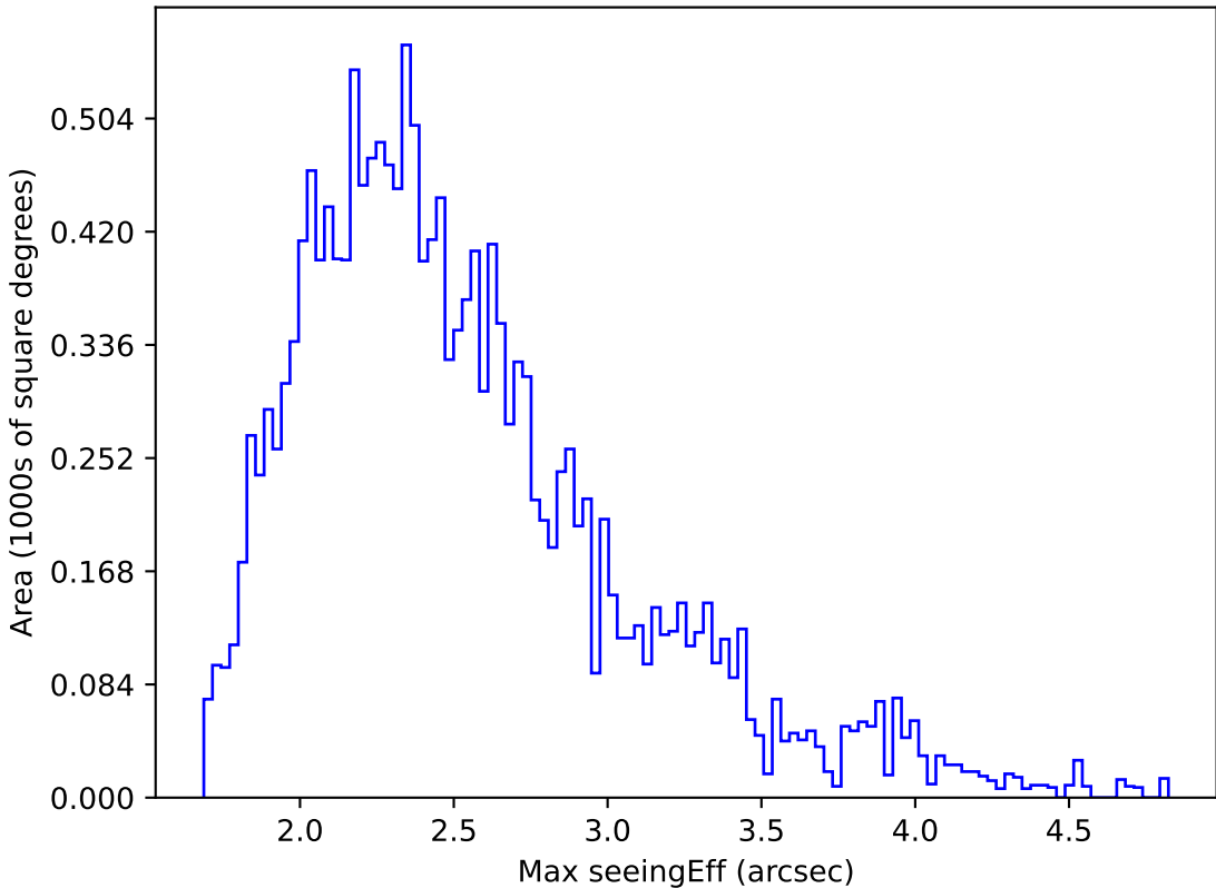
ddf_acor_sf10_lsf20_lsr50_v3.4_10yrs WFD u band: Max seeingEff
