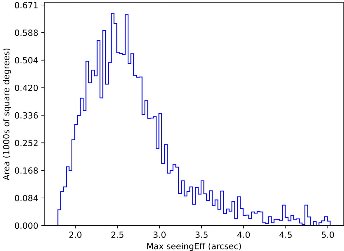
ddf_acor_sf10_lsf20_lsr50_v3.4_10yrs WFD i band: Max seeingEff
