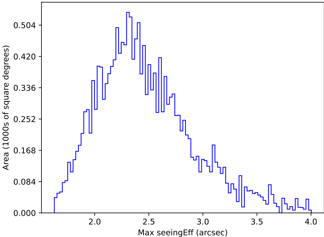
ddf_acor_sf10_lsf20_lsr50_v3.4_10yrs WFD g band: Max seeingEff
