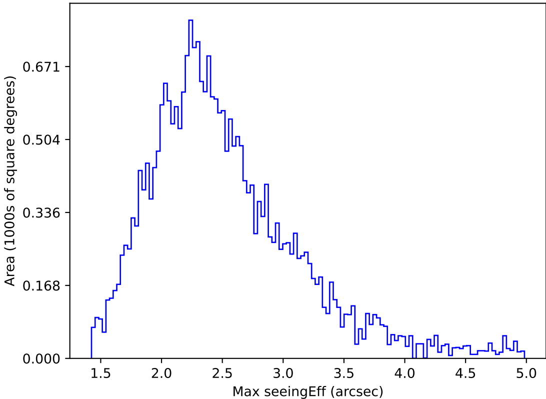
ddf_acor_sf10_lsf20_lsr50_v3.4_10yrs All sky z band: Max seeingEff
