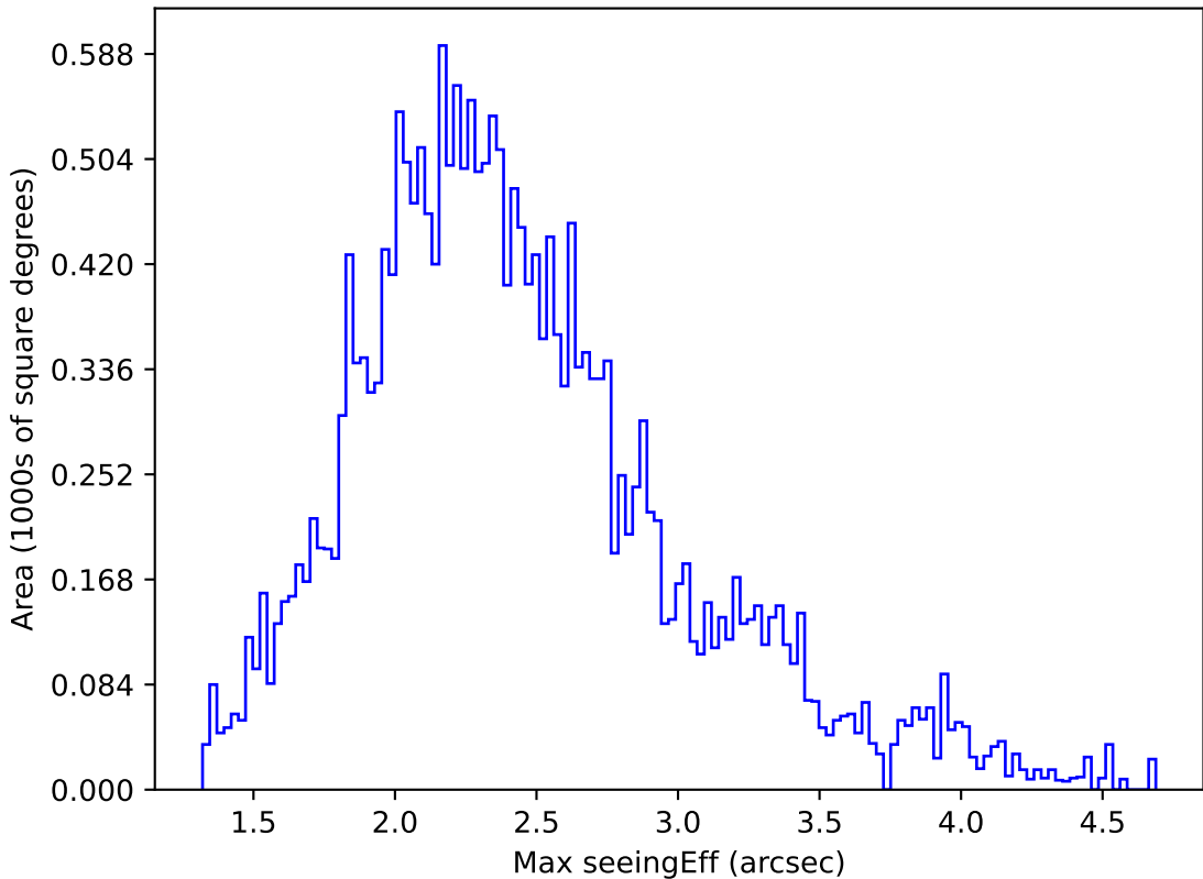
ddf_acor_sf10_ls20_lsr50_v3.4_10yrs All sky u band: Max seeingEff
