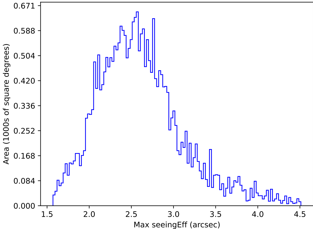
ddf_acor_sf10_lsf20_lsr50_v3.4_10yrs All sky r band: Max seeingEff
