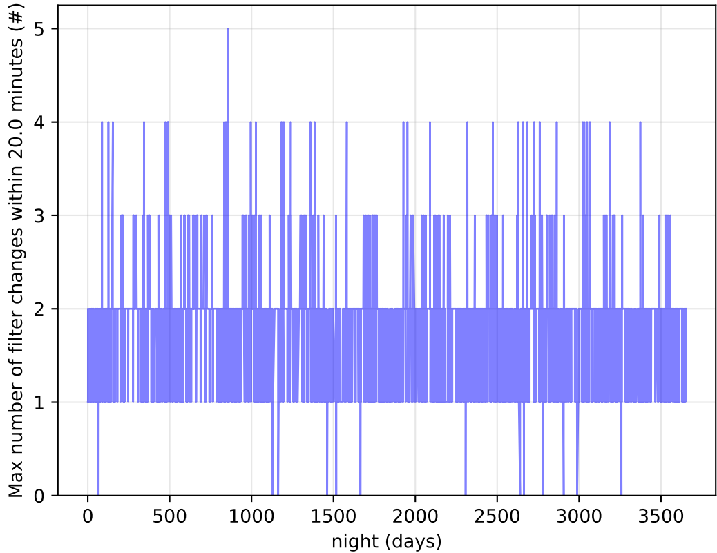
ddf_acor_sf10_Isf20_Isr50_v3.4_10yrs Per Night: Max number of filter changes within 20.0 minutes
